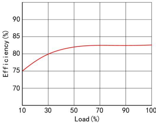
Efficiency/Load graph
