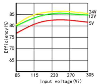
Efficiency/Input voltage graph
