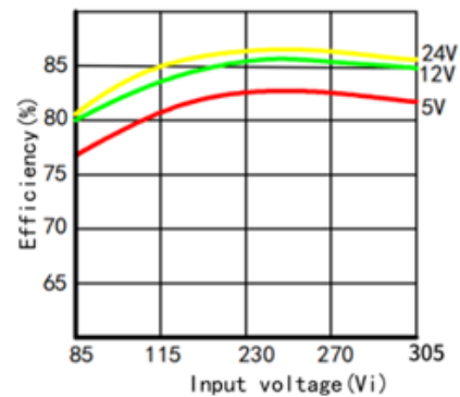
Efficiency/Input voltage graph
