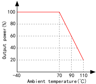
Temperature Curve
