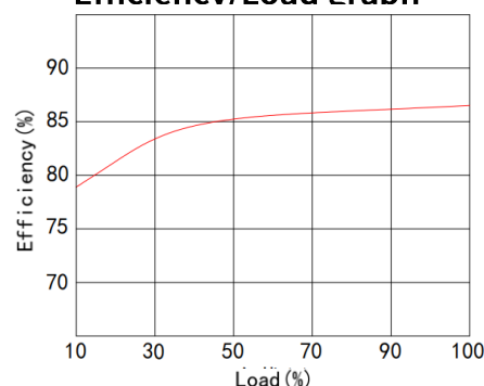
Efficiency/Load graph
