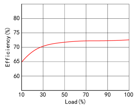
Efficiency/Load graph
