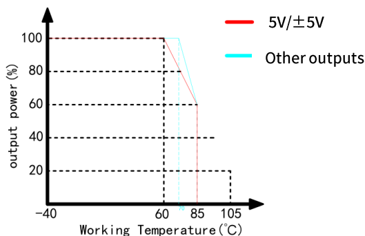
Temperature chart
