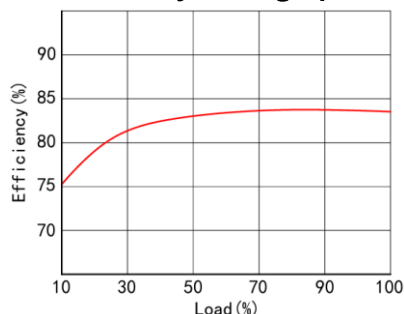
Efficiency/Load graph
