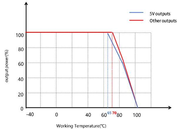
Temperature derating curve (without radiator)
