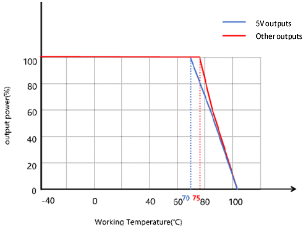
Temperature derating curve (with radiator)
