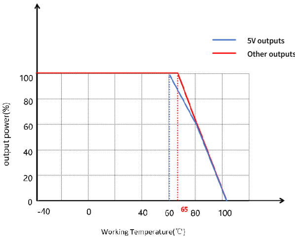
Temperature derating curve (with radiator)
