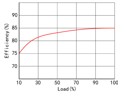
Efficiency/Load graph
