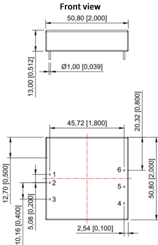
Bottom view
