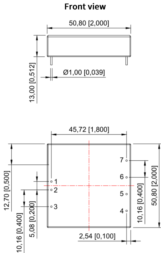
Bottom view
