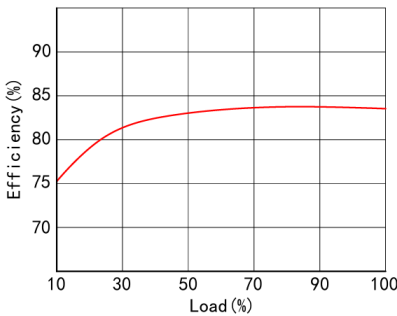
Efficiency/Load graph
