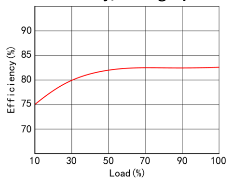
Efficiency/Load graph
