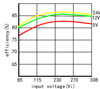
Efficiency/Input voltage graph
