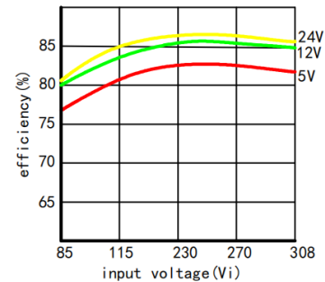
Efficiency/Input voltage graph
